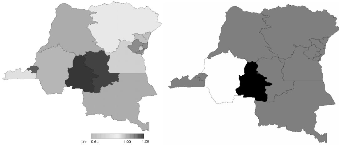
Figure 1: Estimated Odds ratios of residual spatial provincial effects (left) and 95% posterior probability map (right) of child morbidity (CMICS2, 2001).
